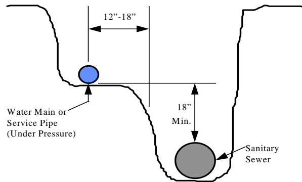
Figure No. 2 - Water Pipe Trenches
